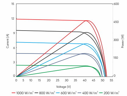
I-V Curves of PV Module (for Ref)
